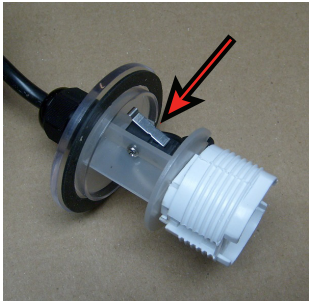
DETAIL OF SAFETY SURFACE MOUNTED SAFETY SWITCH ON ORIGINAL MODELS
